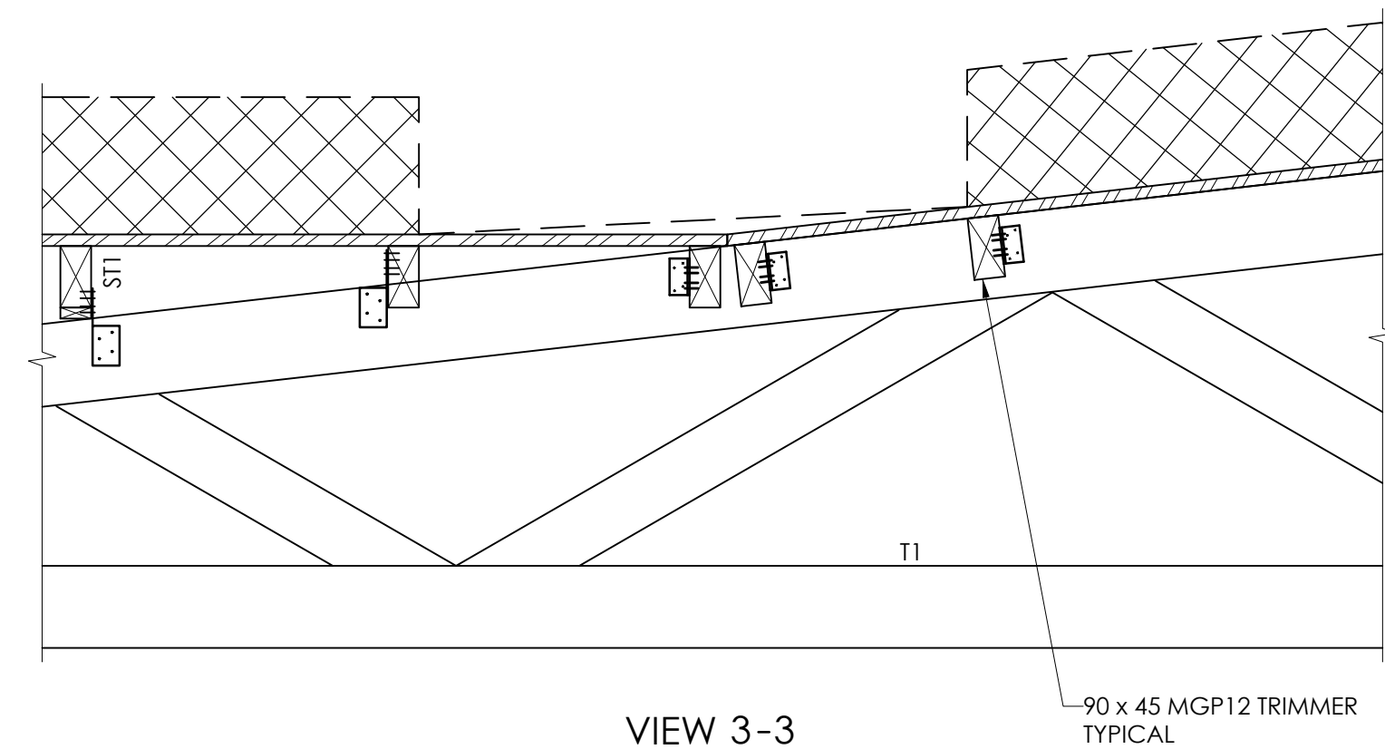
VIEW 3-3
